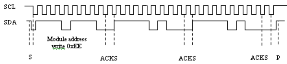
Figure 8: Timing diagram for starting pressure measurement
