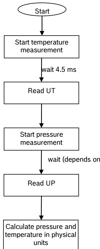
Figure 3: Measurement flow BMP180
