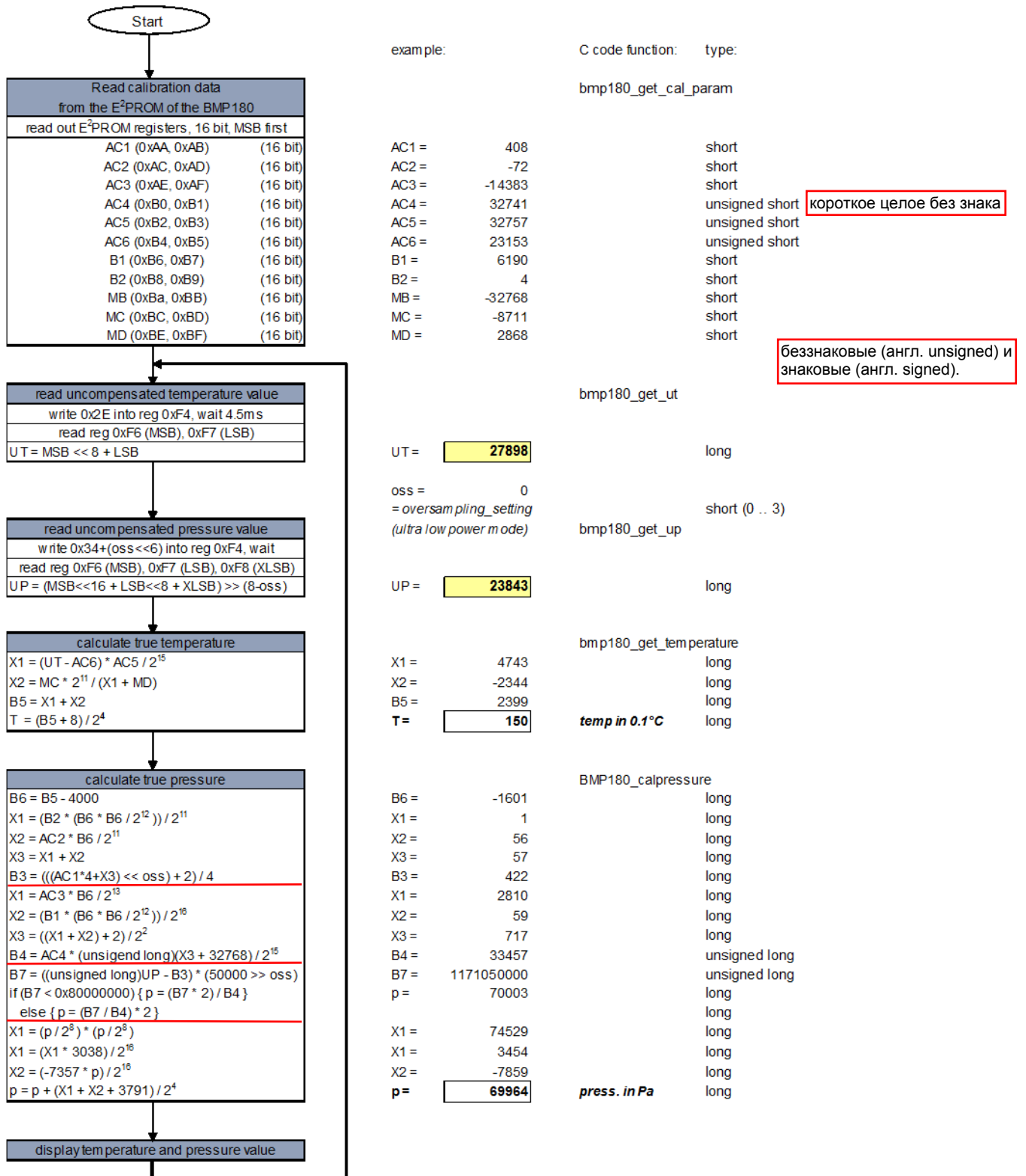
Figure 4: Algorithm for pressure and temperature measurement
